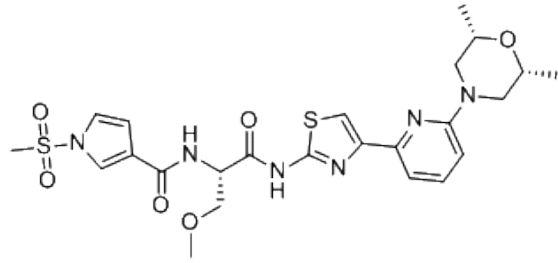
PC-7332001, CDCl 3
